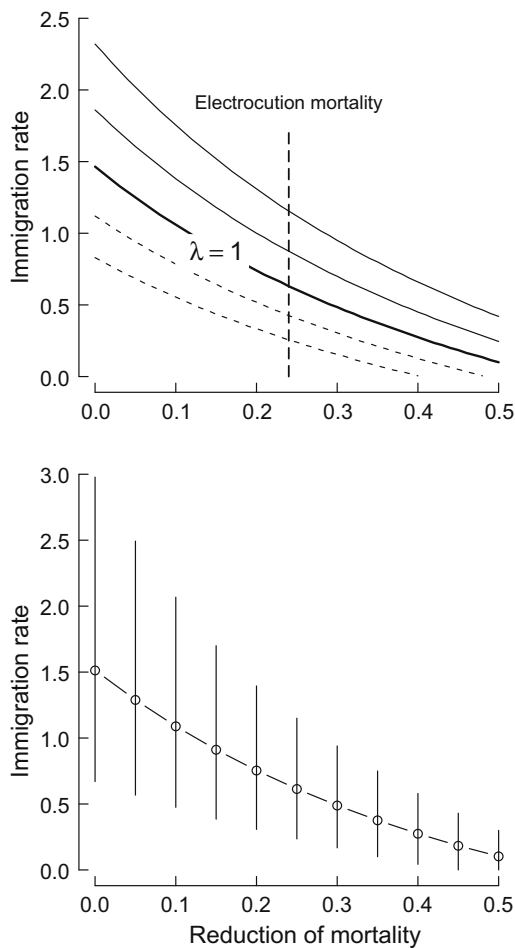
Fig. 4. Relationship between proportional reduction of mortality, immigration rate and population growth rate. Upper panel: the two solid lines represent positive population growth (upper: \lambda = 1.10 , lower: \lambda = 1.05 ), two broken lines negative population growth (upper: \lambda = 0.95 , lower: \lambda = 0.90 ), and the bold line population stability ( \lambda = 1 ). Lower panel: 95% credible intervals of the population growth when it equals 1.
