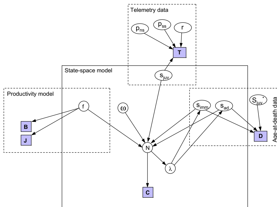
Fig. 1. Directed acyclic graph of the integrated population model used to estimate demographic parameters of eagle owls. Data are symbolized by grey rectangles, parameters by ellipses, the relationship between them by arrows and sub-models by open rectangles. Notation: T: telemetry data; D: age-at-death data; C: population survey; B: number of surveyed broods for assessing reproductive success; J: annual number of fledglings; S_{juv} : apparent juvenile survival; S_{imm} : immature survival; S_{ad} : adult survival; S_{juv}^* : juvenile survival; \omega : immigration rate; f : productivity; N : population size; \lambda : population growth rate; p_{ns} : reencounter rate after preceding encounter failure; p_{ss} : reencounter rate after preceding encounter; r : probability to find a freshly dead individual. Note that the priors are excluded from this graph to increase visibility.
