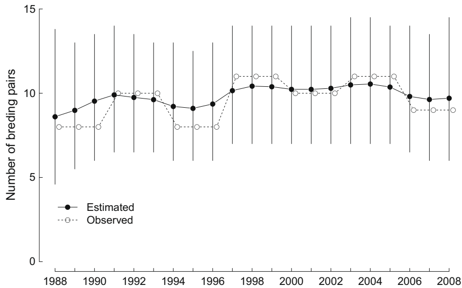
Fig. 2. Estimated (posterior mean and 95% credible intervals) and observed population sizes of the eagle owl population in Valais, southwestern Swiss Alps.
