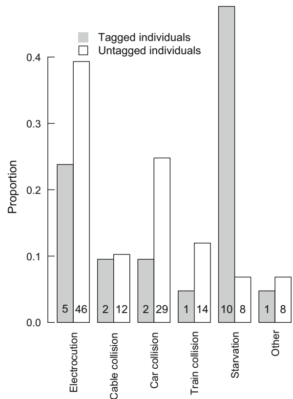
Fig. 3. Proportion of mortality causes of 21 tagged and 117 untagged (incidentally found) eagle owls. Starvation refers to natural mortality, with all other mortality causes being anthropogenic. The figures at bar foot indicate sample size.
